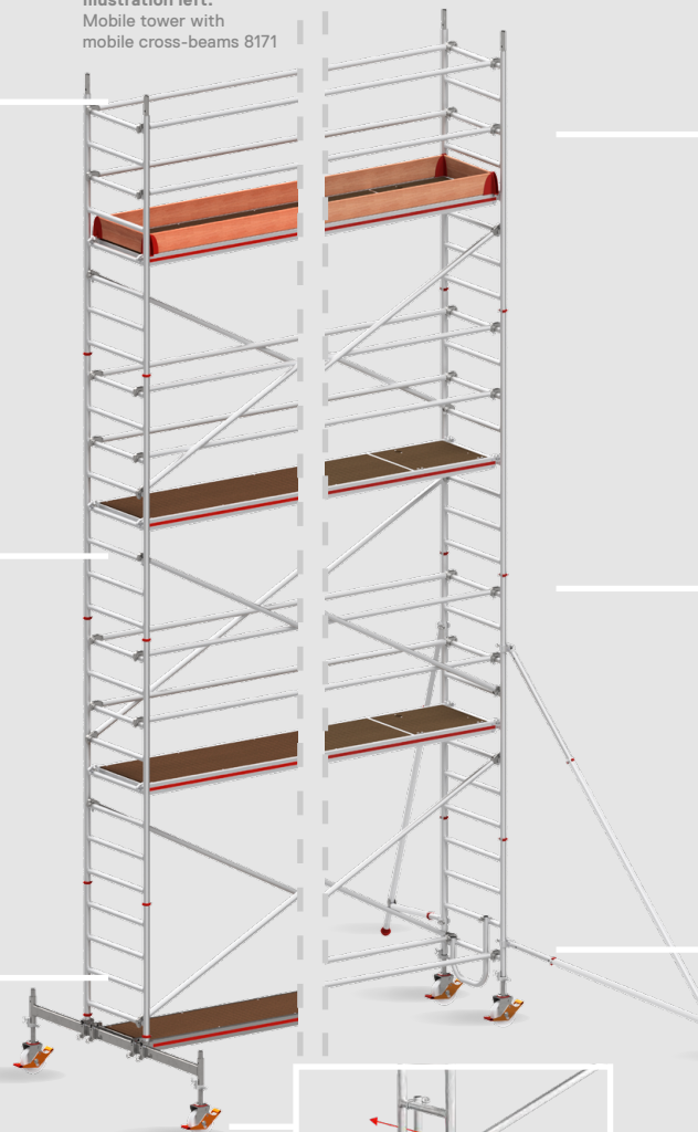
Illustration right: Mobile tower with stabilisers 8371
